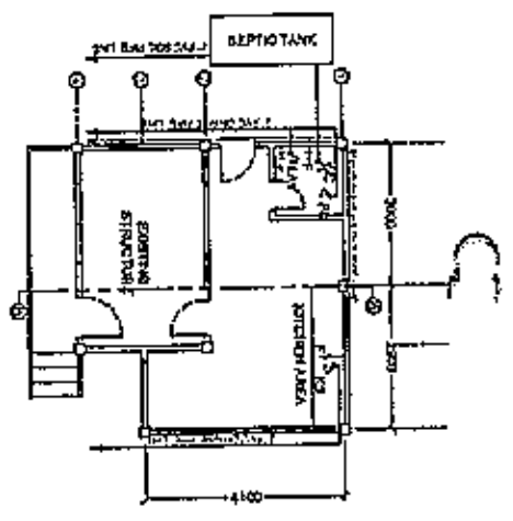
PLUMBING LAYOUT
