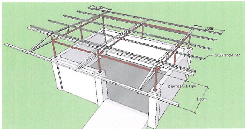
STEEL FURLINS DIMENSIONS
