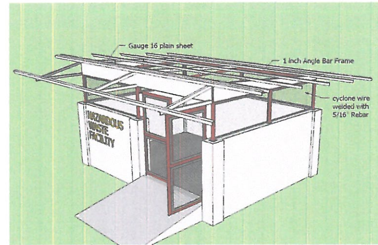
GATE AND ROOFING SPECIFICATIONS
