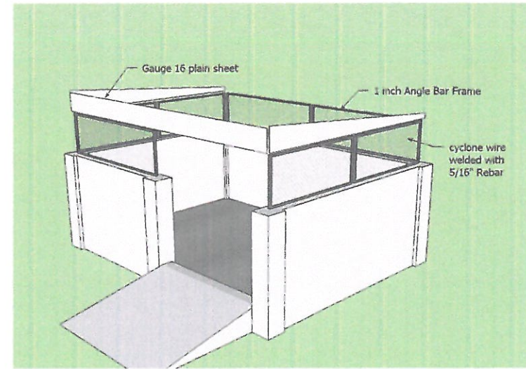
SCREEN VENTILATION
