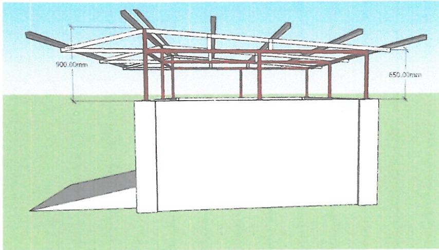
ROOFING HEIGHT DIMENSIONS
